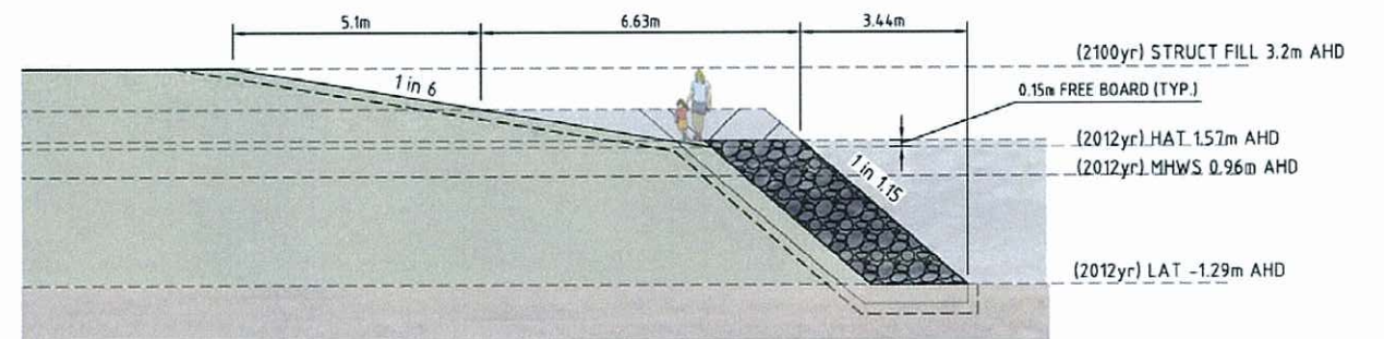
Lowest Astronomical Tide Option (Seawall Base Level)
